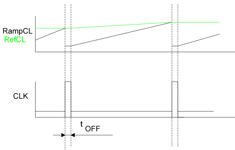
Figure 10: clock modulation
